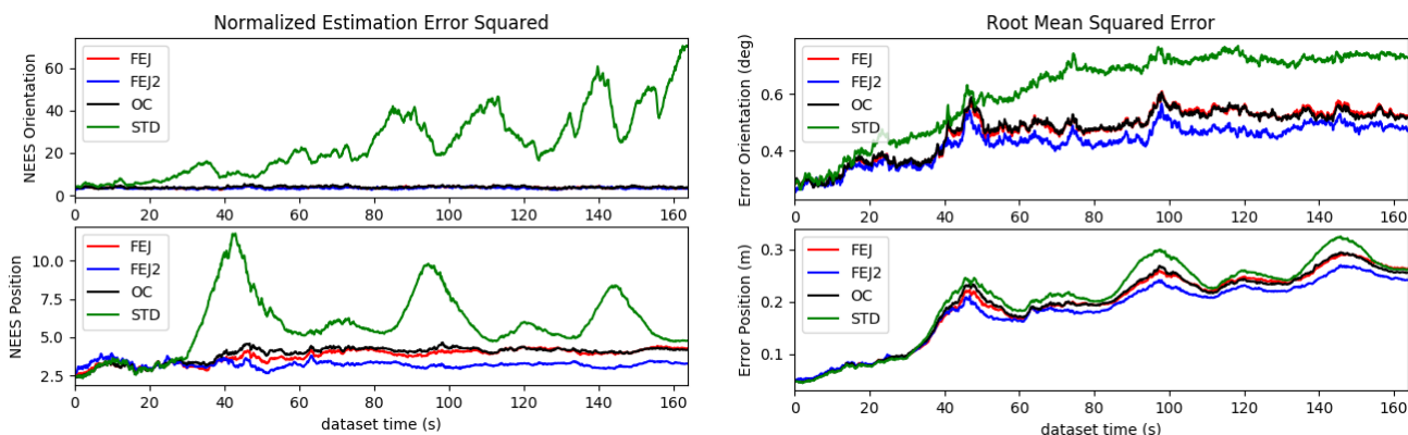
Fig. 2: The average RMSE and NEES over 50 Monte-Carlo simulation for IMU orientation and position with stereo measurements and 2 pixel noises.
